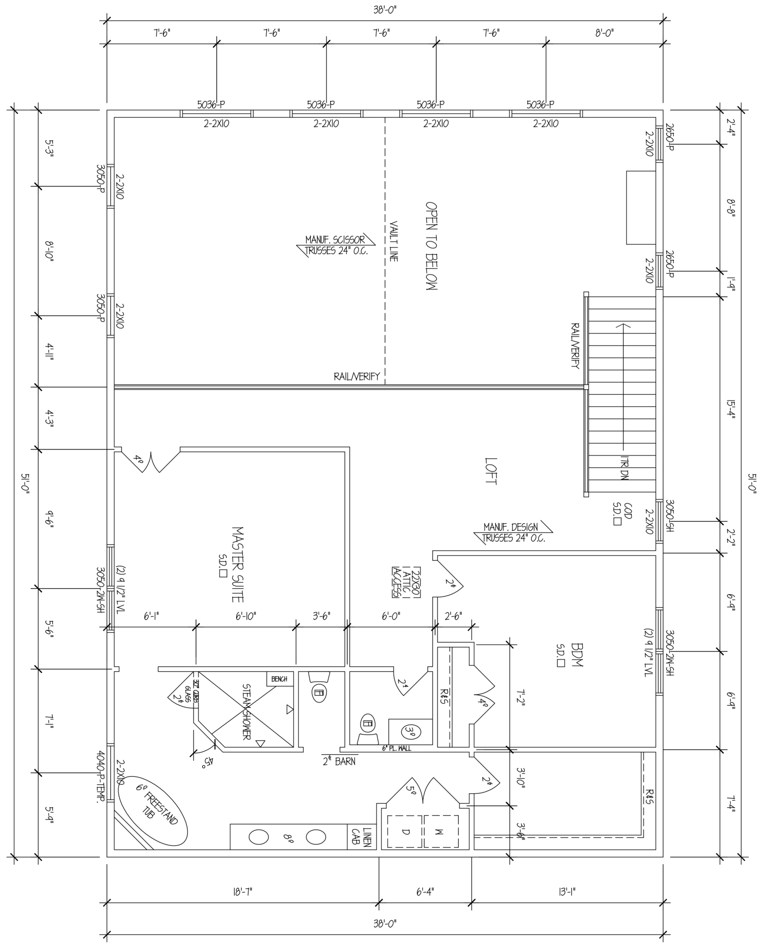
1 UPPER LEVEL 1938 S.F. A4 1/4"=1'-0"
