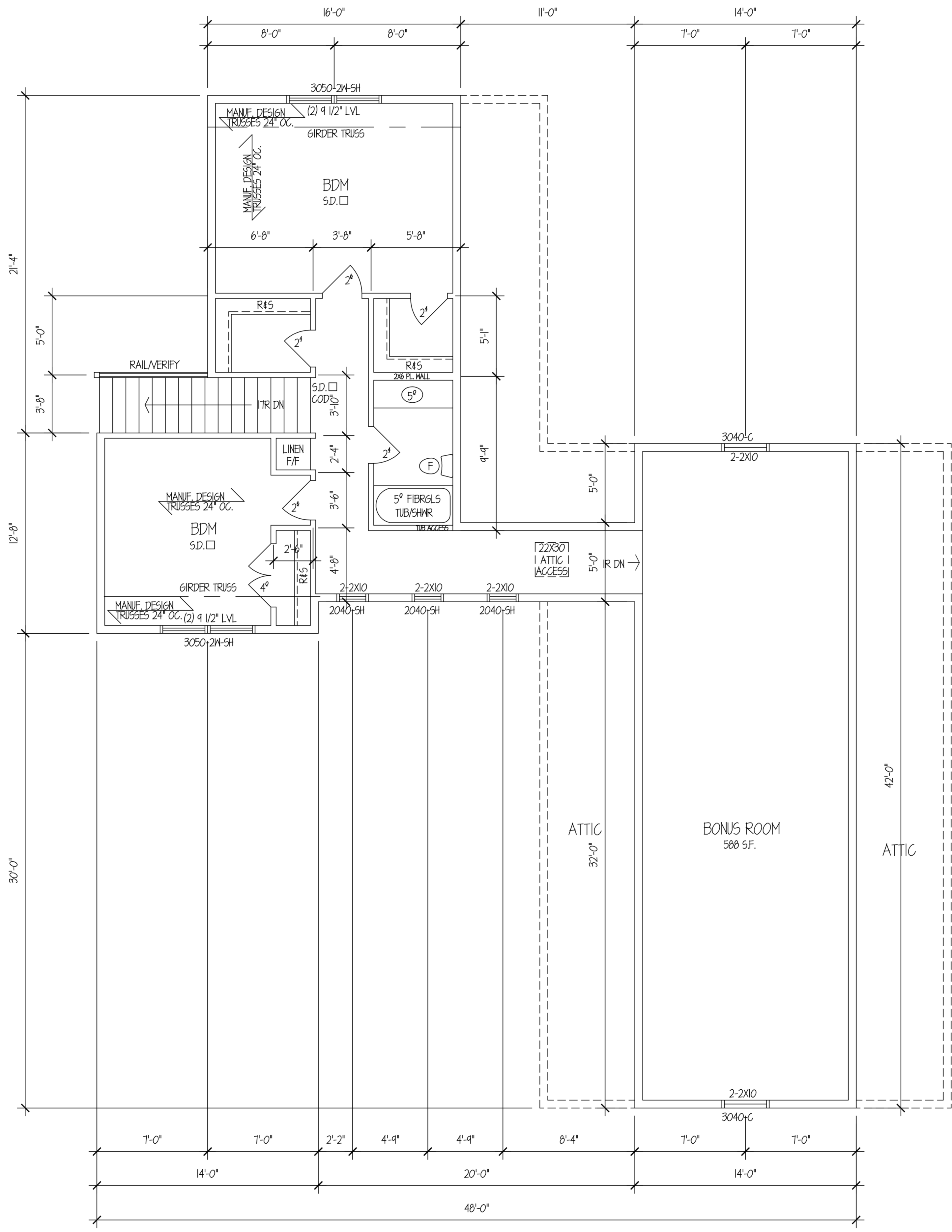
1 UPPER LEVEL 644 S.F. A4 1/4"=1'-0"
