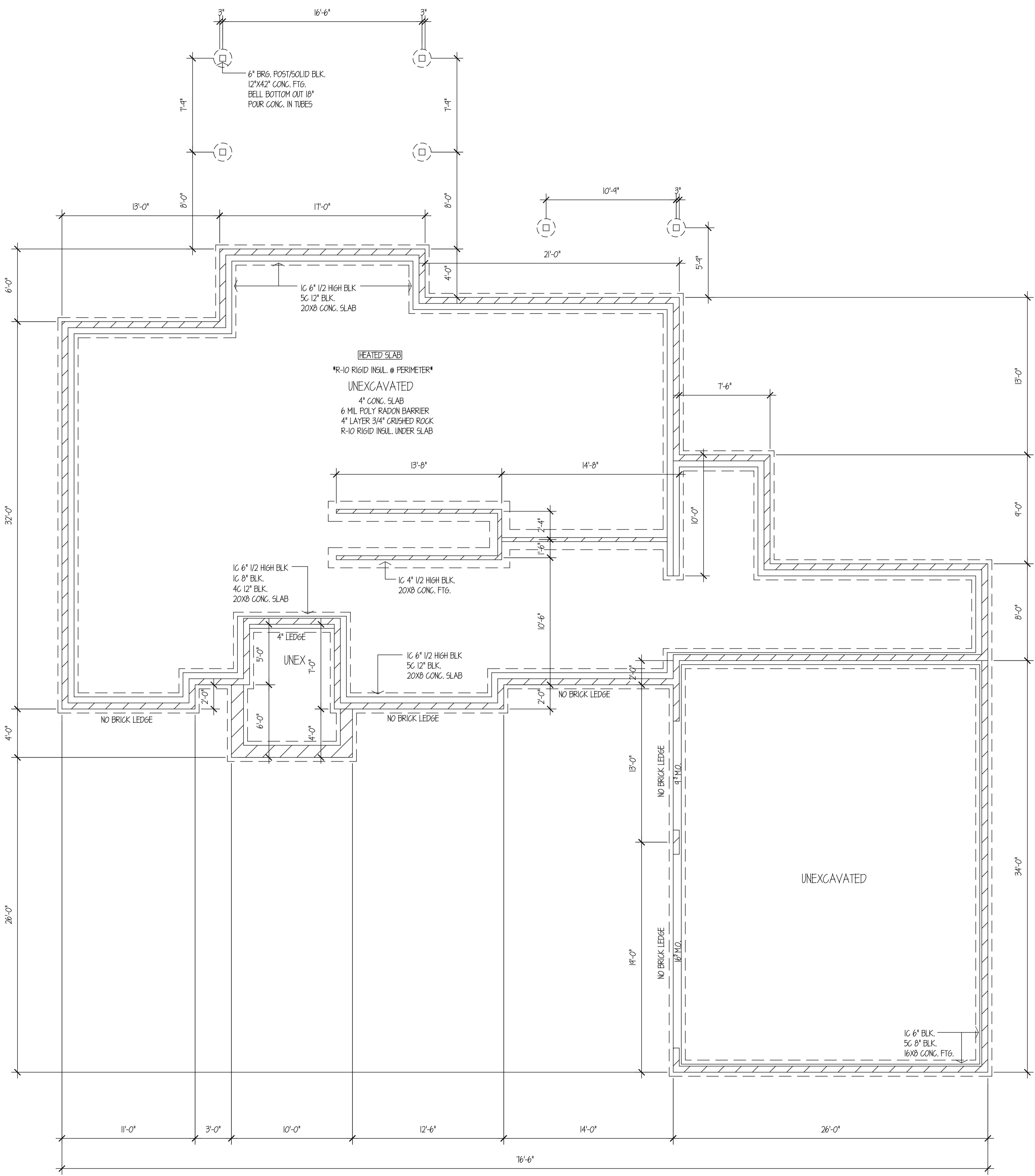
1 FOUNDATION PLAN A2 1/4"=1'-0"
